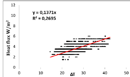
Figure 5 The heat flux and temperature difference measured at the foam glass case study house
