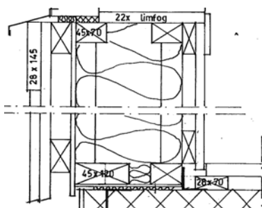
Figure 1 Case study of detached house with wood fibre insulation material
