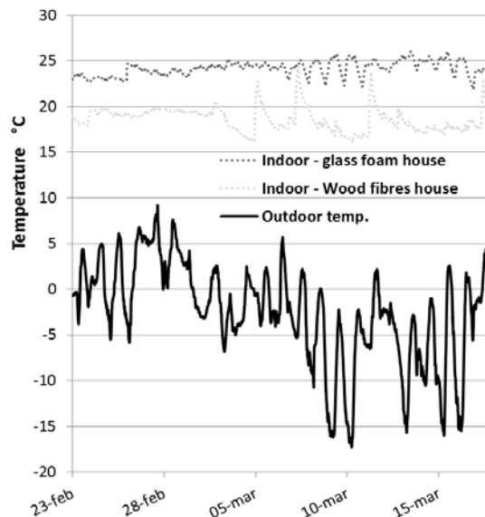
Figure 3 Measurements of the indoor and outdoor temperatures
