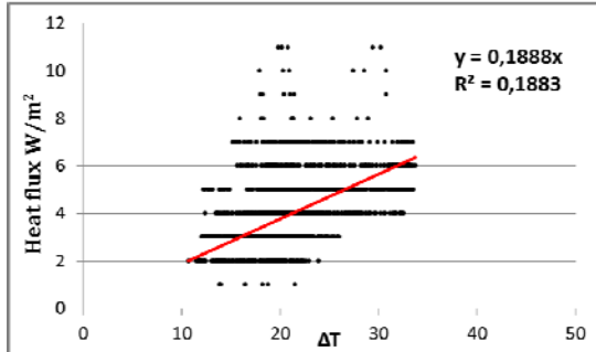
Figure 4 The heat flux and temperature difference measured at the wood fibre case study house
