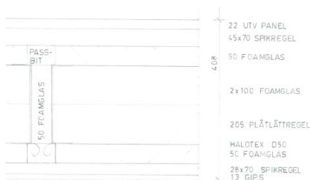
Figure 2 Case study of detached house with foam glass insulation material
